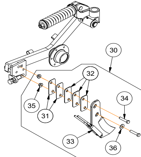
Dual Injector Knife
