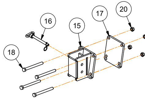
Outer Wing Gauge Wheel
