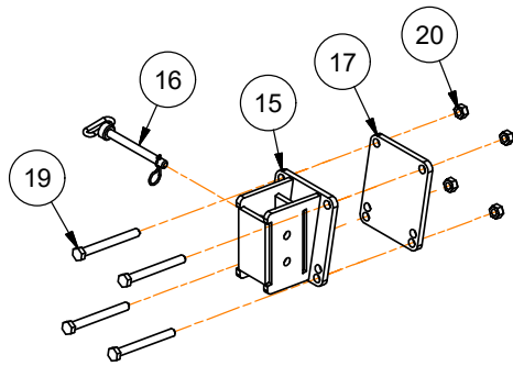
Main Wing Gauge Wheel
